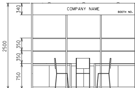
ELEVATION 3M(W) X 3M(D) X 2.5M(H) Left Corner Booth A
