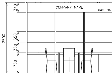
ELEVATION 3M(W) X 3M(D) X 2.5M(H) Right Corner Booth A
