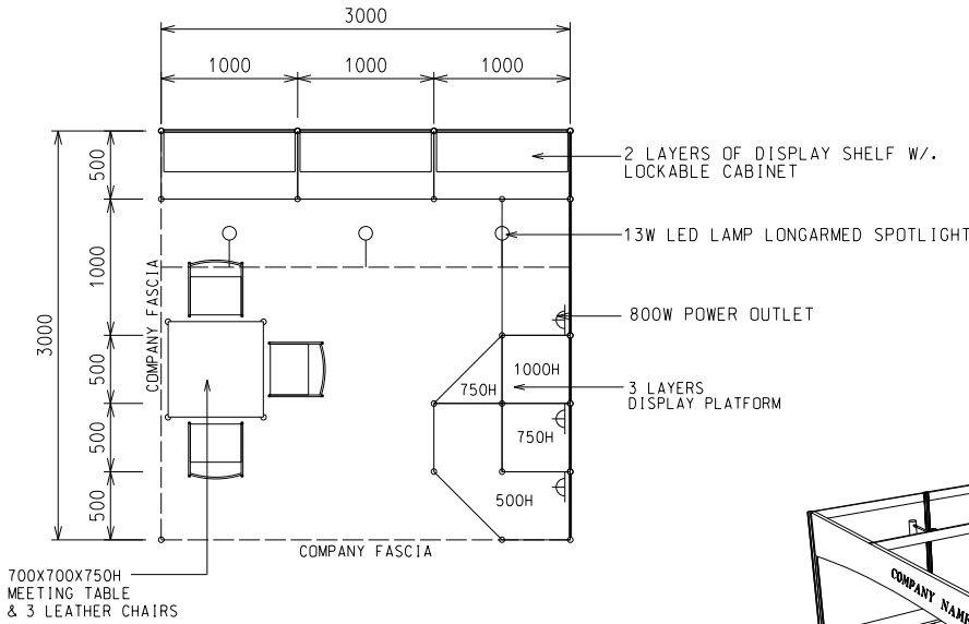
PLAN 3M(W) X 3M(D) X 2.5M(H) Left Corner Booth B
