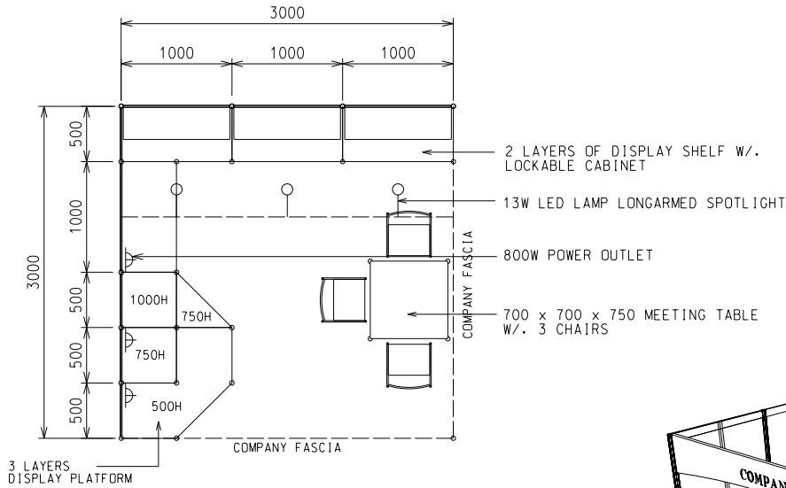
PLAN 3M(W) X 3M(D) X 2.5M(H) Right Corner Booth B
