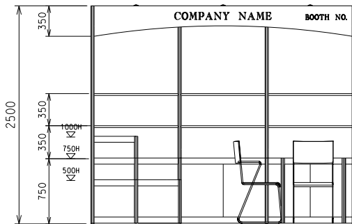
ELEVATION 3M(W) X 3M(D) X 2.5M(H) Right Corner Booth B
