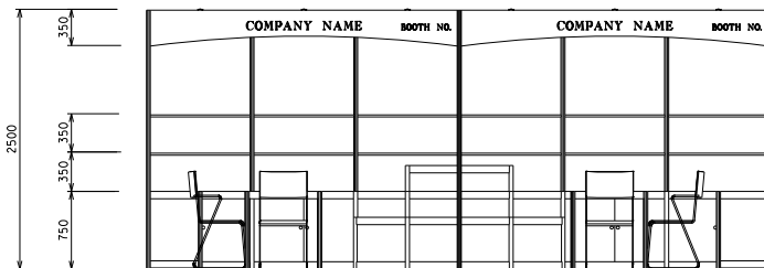
ELEVATION 6M(W) X 3M(D) X 2.5M(H) LEFT CORNER BOOTH B
