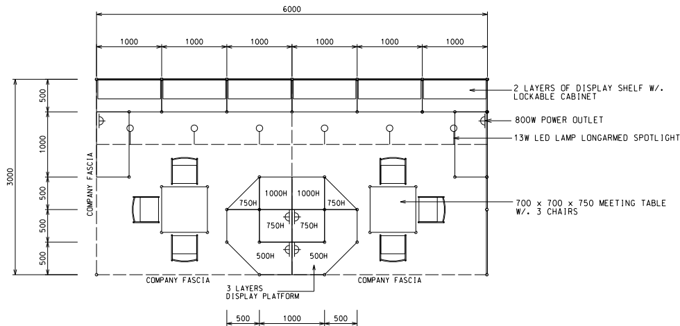
PLAN 6M(W) X 3M(D) X 2.5M(H) LEFT CORNER BOOTH B
