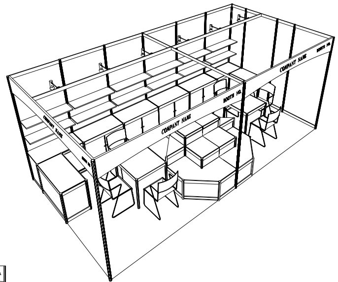
PERSPECTIVE 6M(W) X 3M(D) X 2.5M(H) LEFT CORNER BOOTH B
