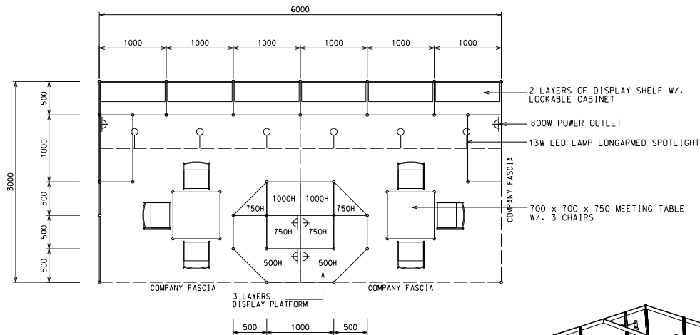
PLAN 6M(W) X 3M(D) X 2.5M(H) RIGHT CORNER BOOTH B
