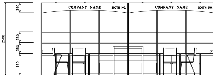
ELEVATION 6M(W) X 3M(D) X 2.5M(H) RIGHT CORNER BOOTH B
