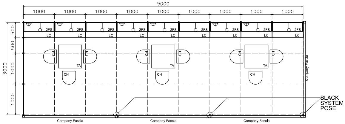
PLAN
